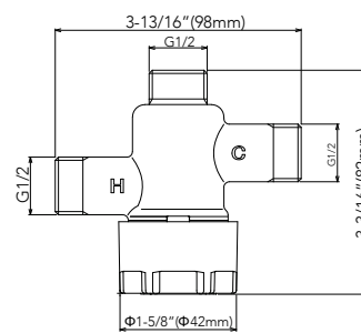
Thermostatic Mixing Valve (TLT10R)
